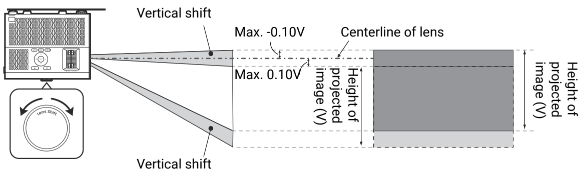
Ceiling mount-front projection
